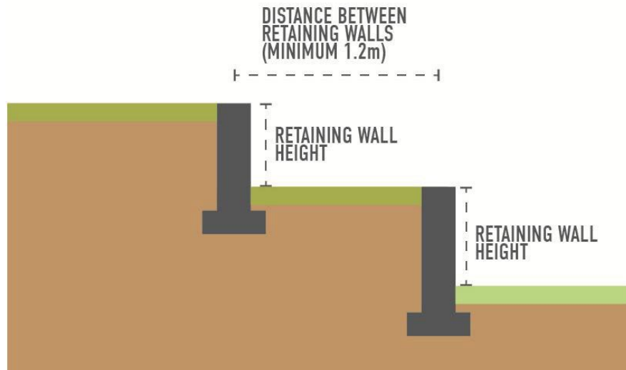
Figure 7-2. Retaining Walls
