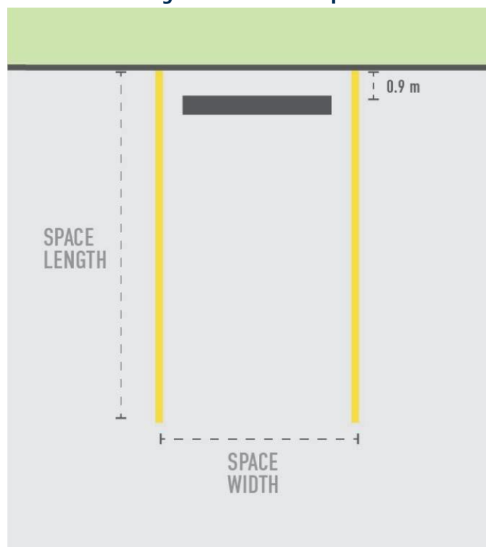
Figure 8-2. Wheel Stops
