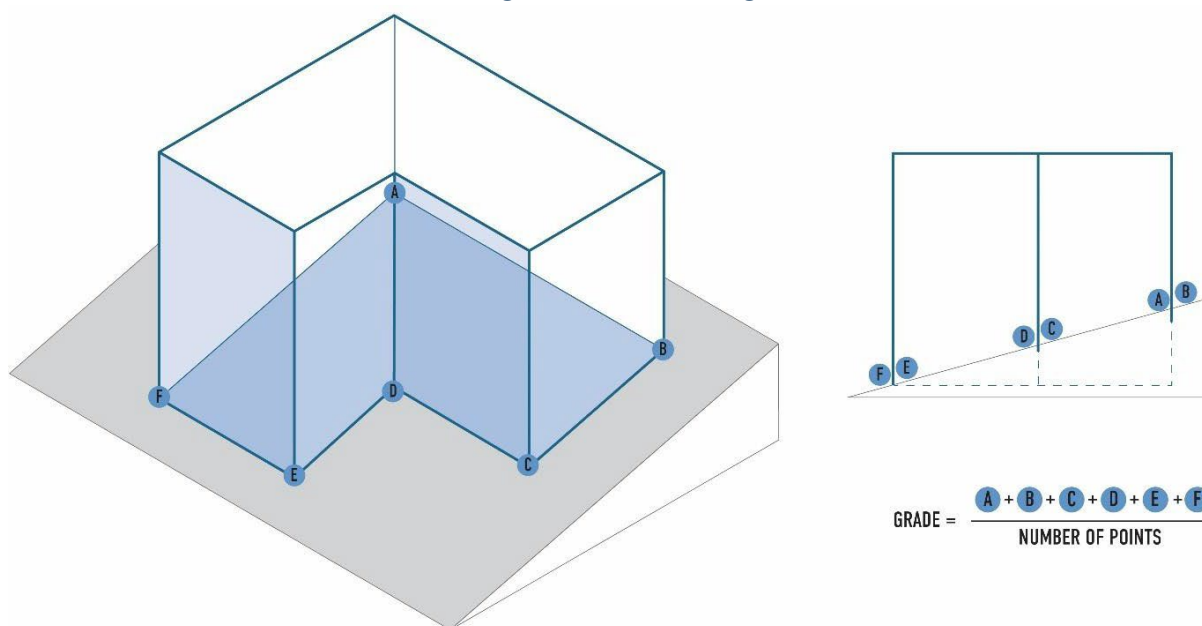
Figure 5-1. Calculating Grade
