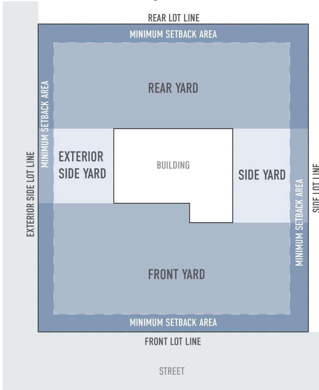
Figure 4-7. Yards
