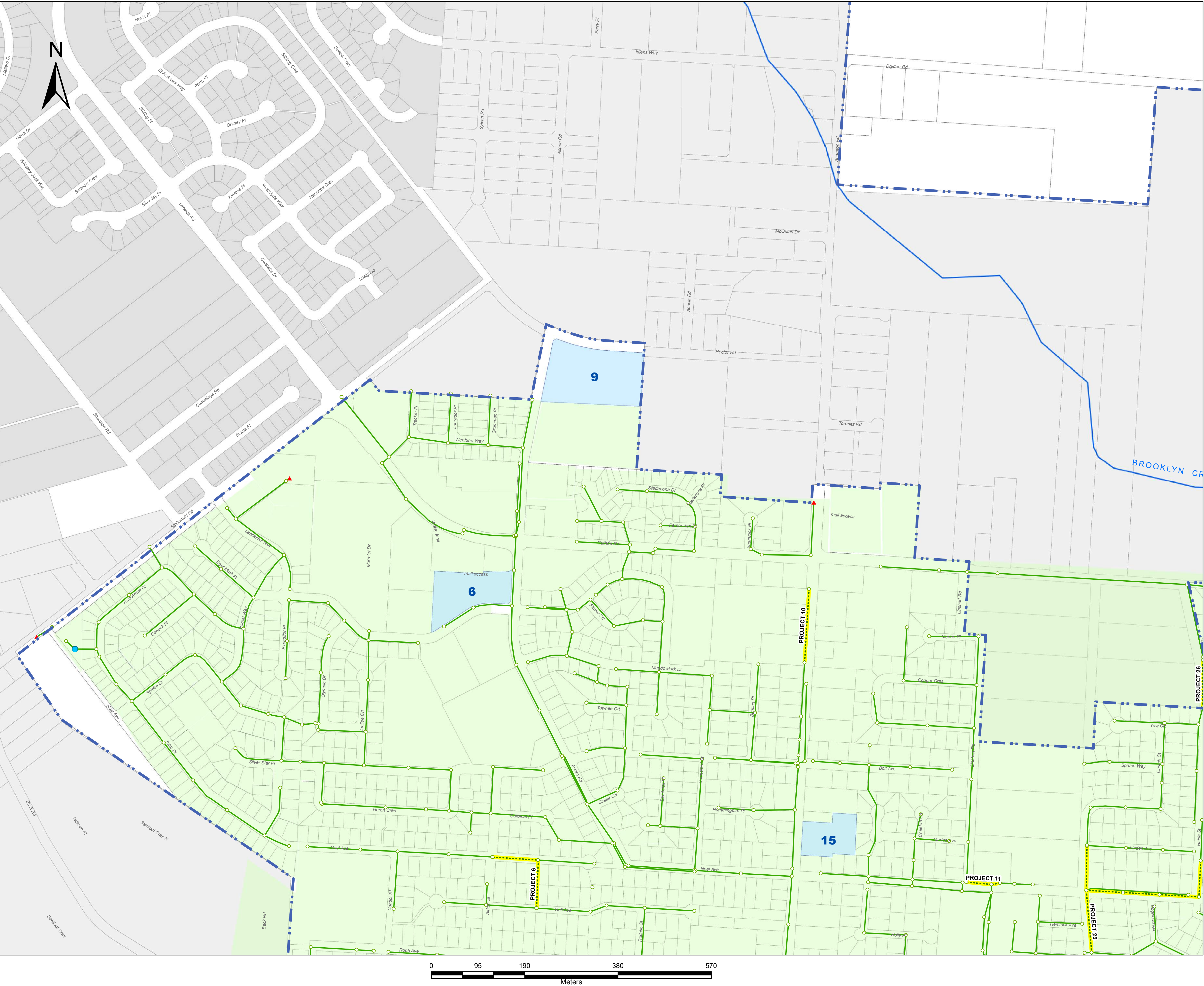
Fig - 5A LTF (20yr) Growth Nodes and Proposed Drainage Improvement Projects NW QUADRANT 2013 Storm Drainage Model Update
