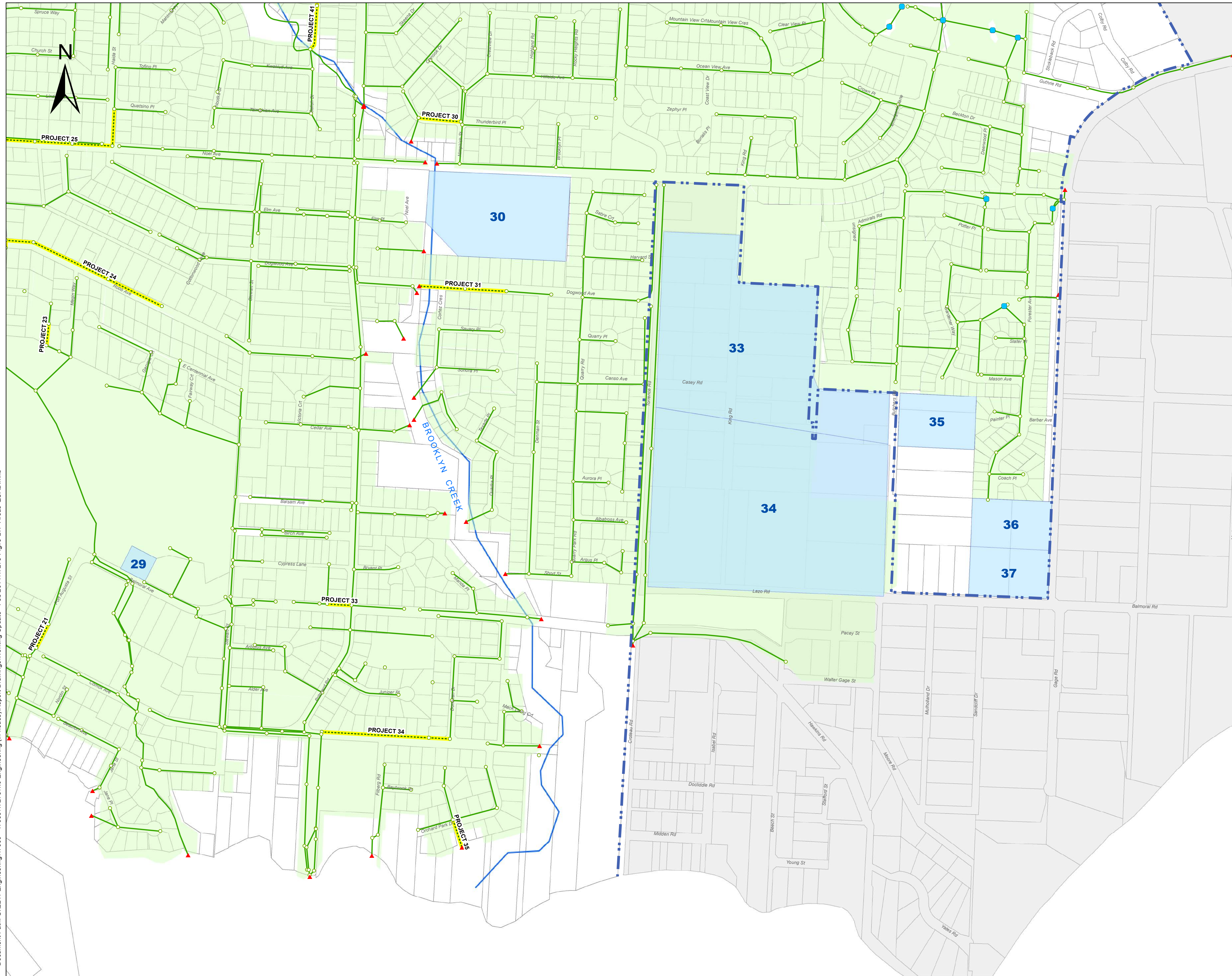
Fig - 5D LTF (20yr) Growth Nodes and Proposed Drainage Improvement Projects SE QUADRANT 2013 Storm Drainage Model Update
