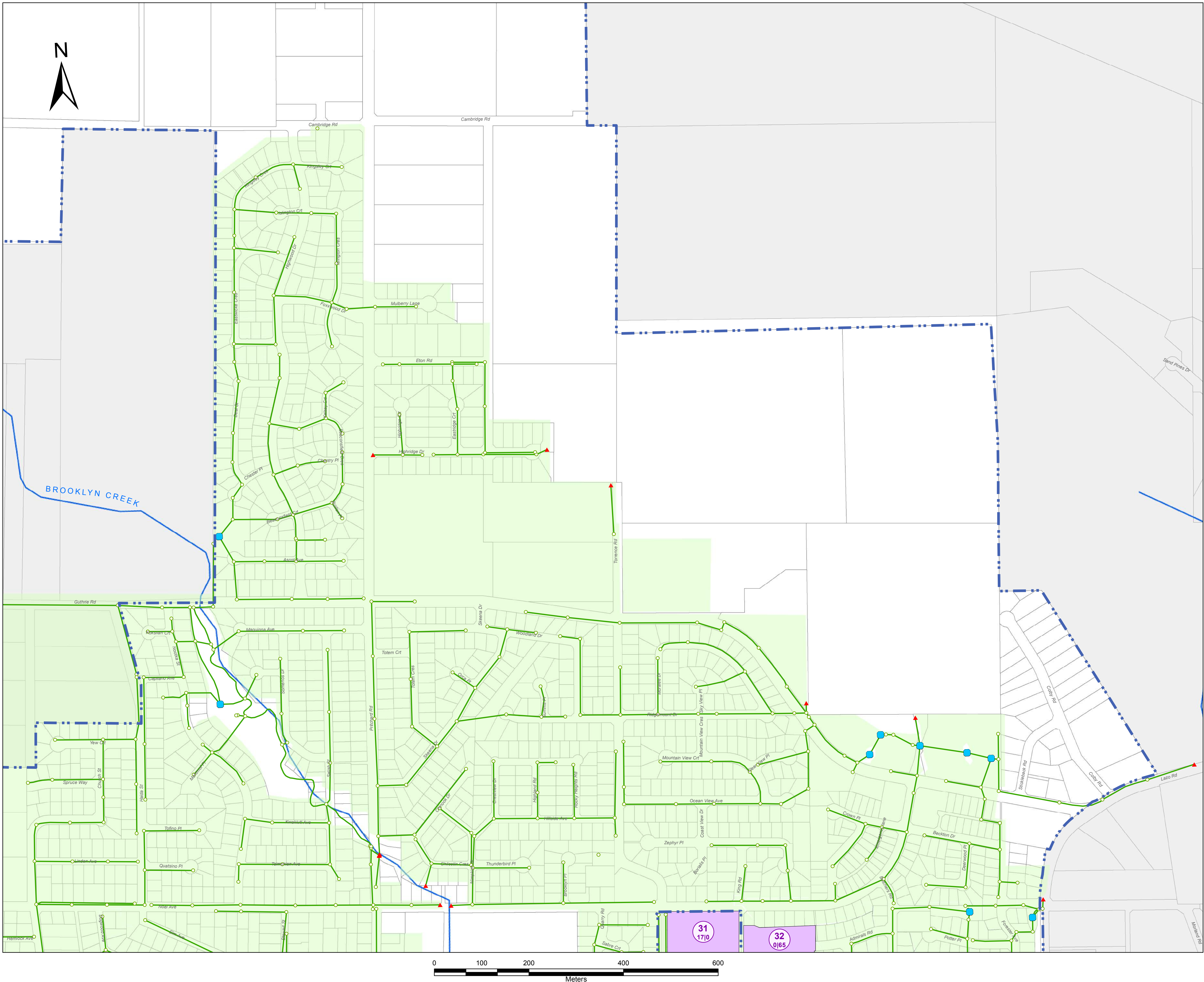
Fig - 4B STF (5yr) Growth Nodes and Proposed Drainage Improvement Projects NE QUADRANT
