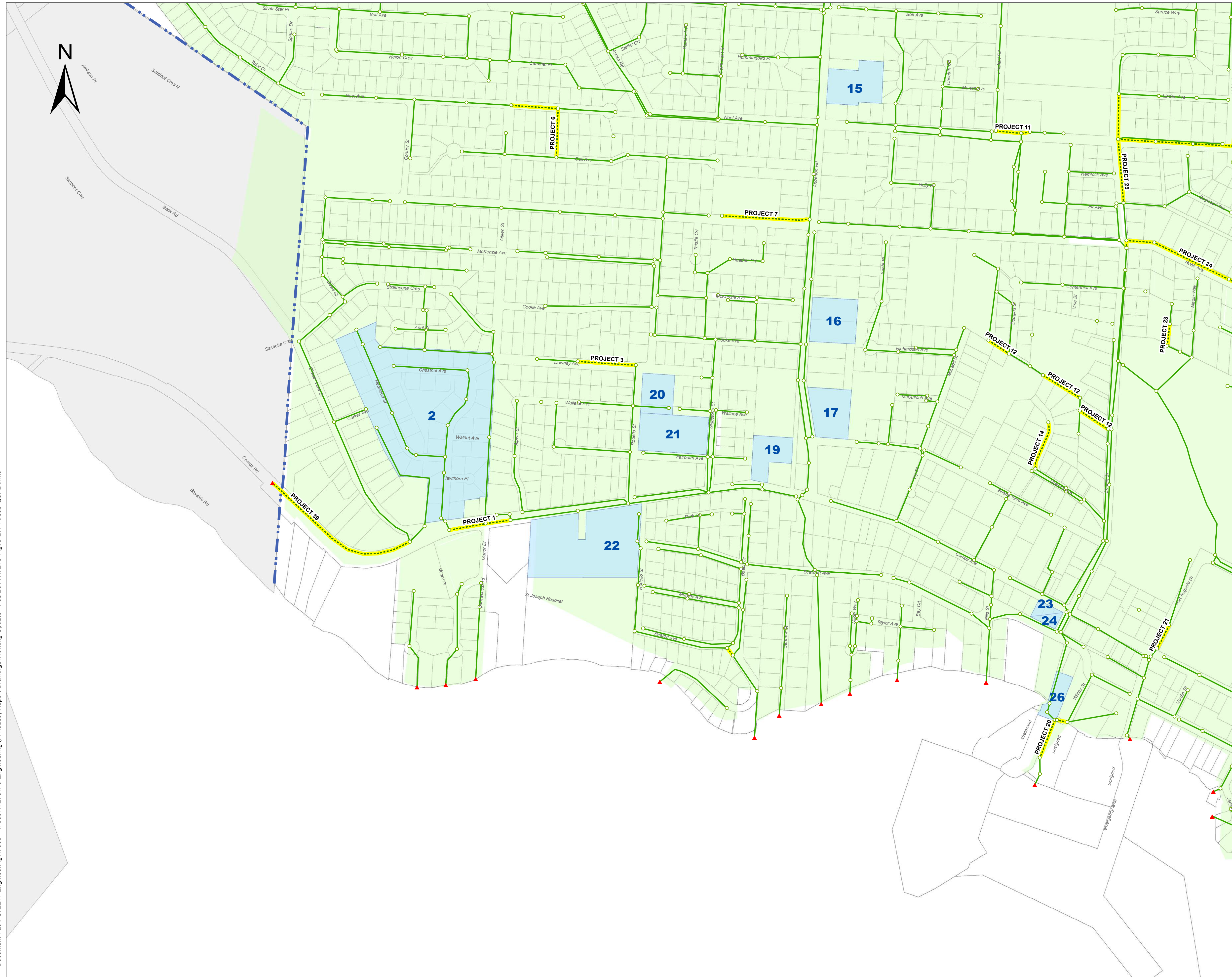
Fig - 5C LTF (20yr) Growth Nodes and Proposed Drainage Improvement Projects SW QUADRANT 2013 Storm Drainage Model Update
