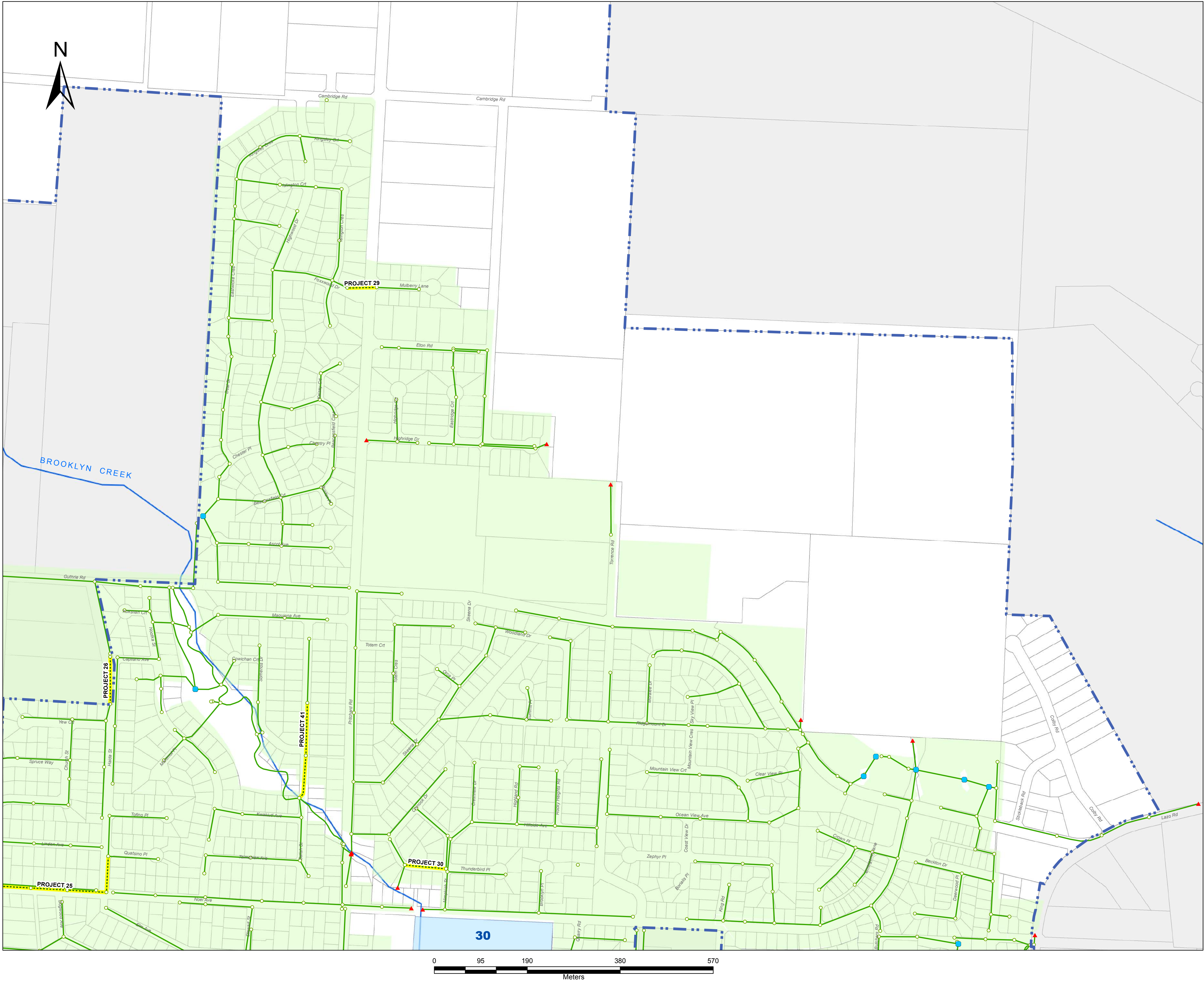
Fig - 5B LTF (20yr) Growth Nodes and Proposed Drainage Improvement Projects NE QUADRANT 2013 Storm Drainage Model Update
